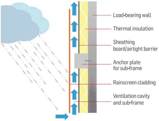
Diagram A Fixing system for solid-wall construction
