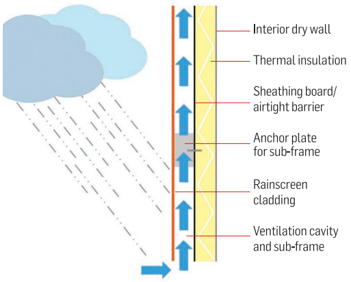
Diagram B Fixing system for modular construction
