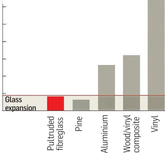
Figure 4: Comparison of expansion and contraction of various materials
