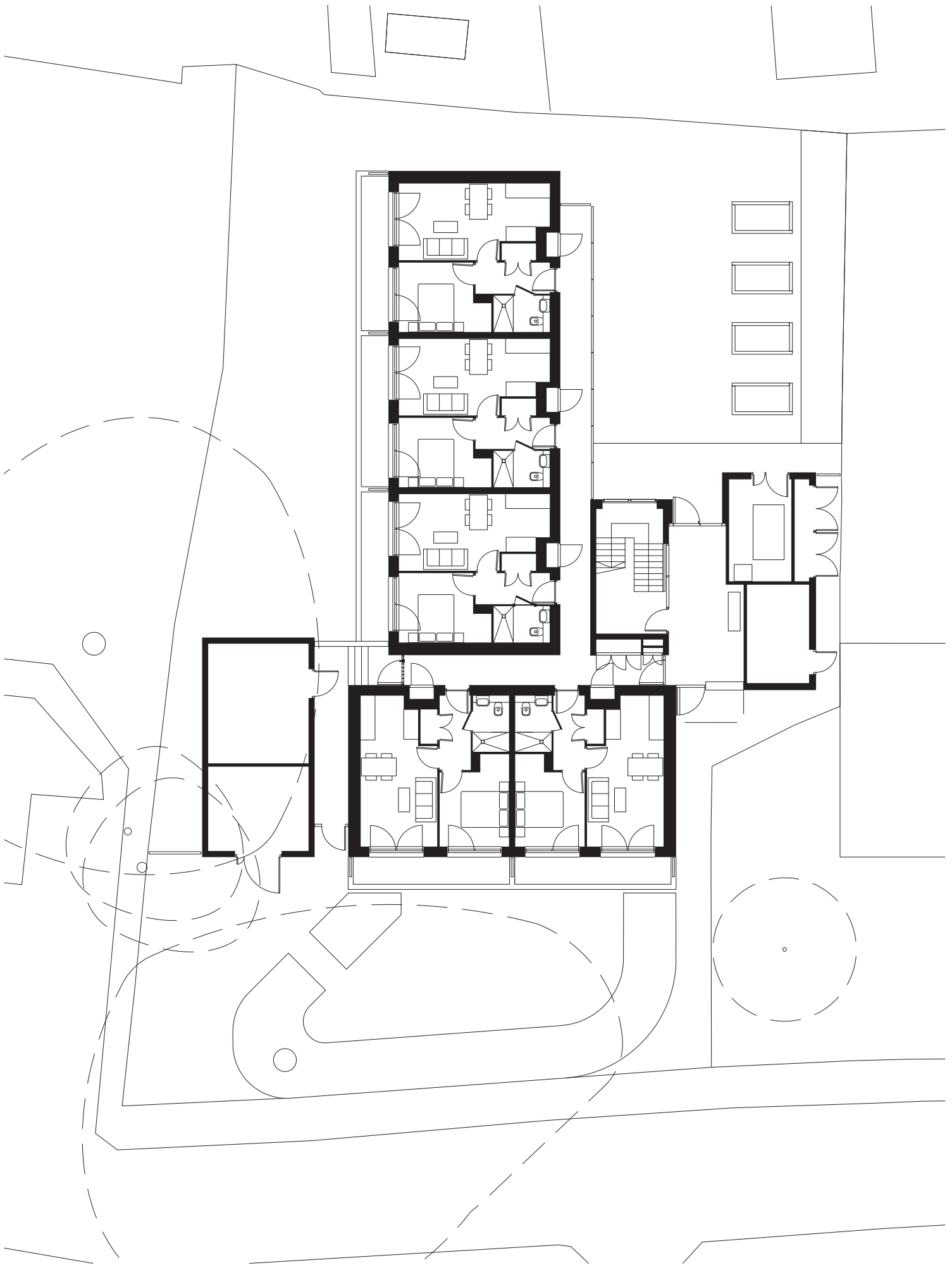
Gardner Close: Ground Floor Plan
