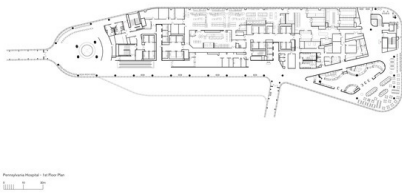
Project Name Penn Patient Pavilion, University of Pennsylvania Filename 2349_FP780742.pdf Copyright holder Foster + Partners Caption Drawing - 1st floor plan
