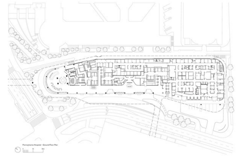
Project Name Penn Patient Pavilion, University of Pennsylvania Filename 2349_FP780741.pdf Copyright holder Foster + Partners Caption Drawing - ground floor plan
