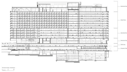
Project Name Penn Patient Pavilion, University of Pennsylvania Filename 2349_FP780747.pdf Copyright holder Foster + Partners Caption Drawing - section
