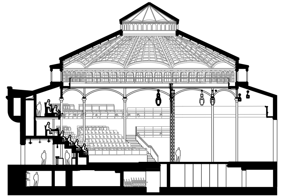
Flat Floor Format Plant scengolv
