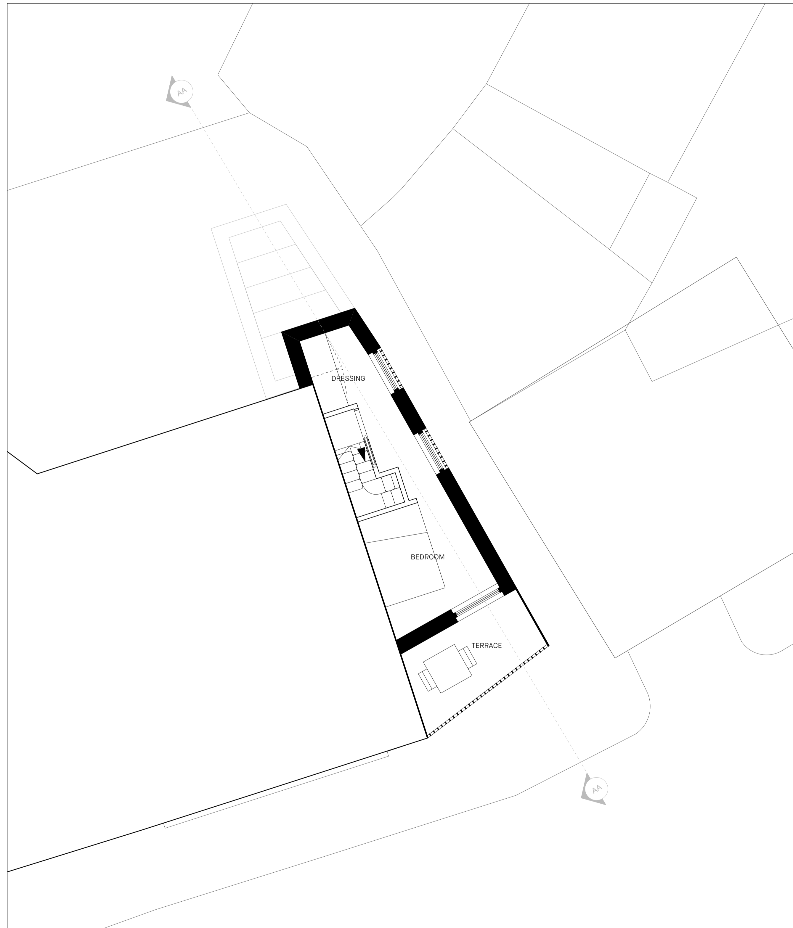
Proposed Second Floor Plan Scale: 1:50
