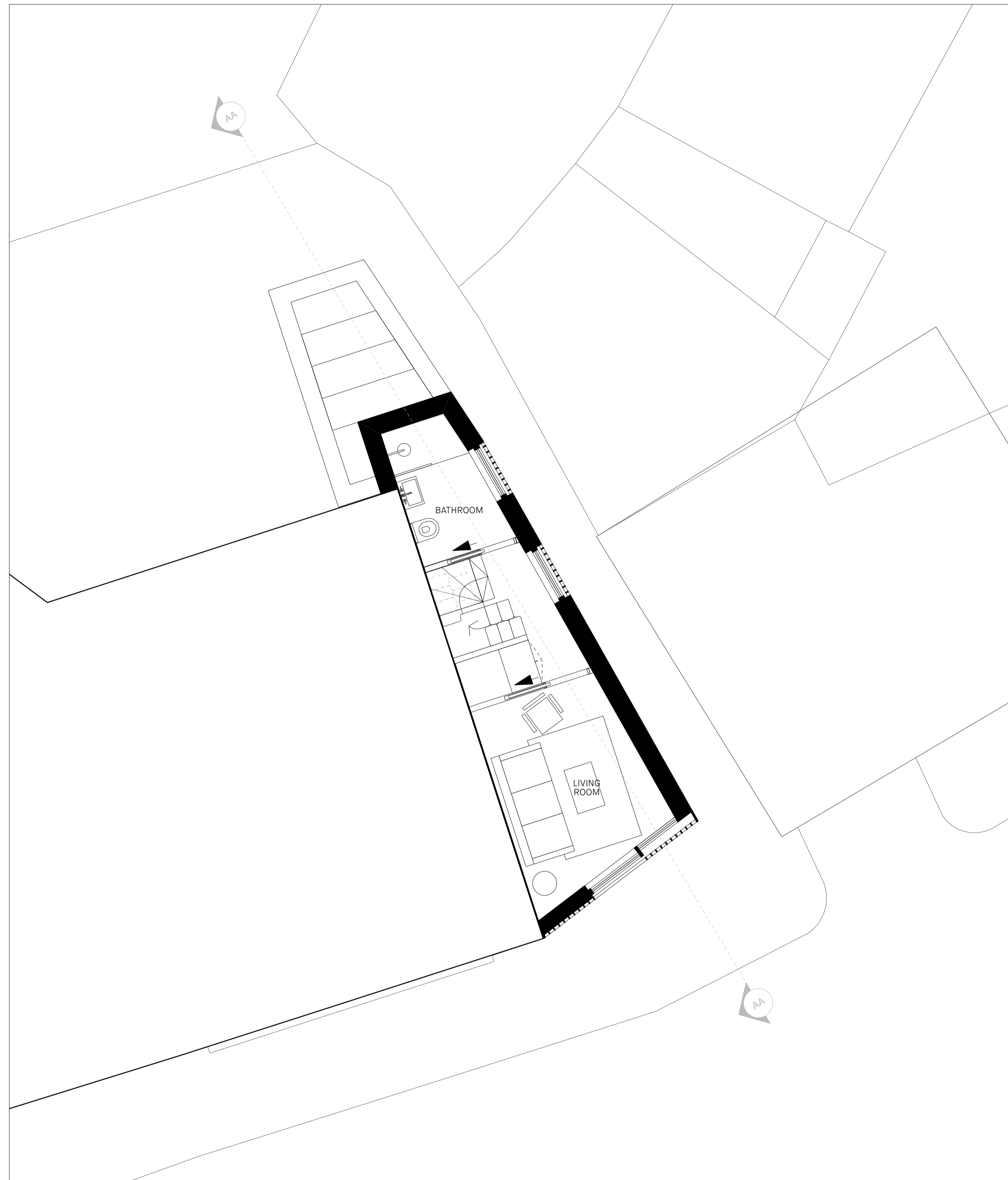
Proposed First Floor Plan Scale: 1:50
