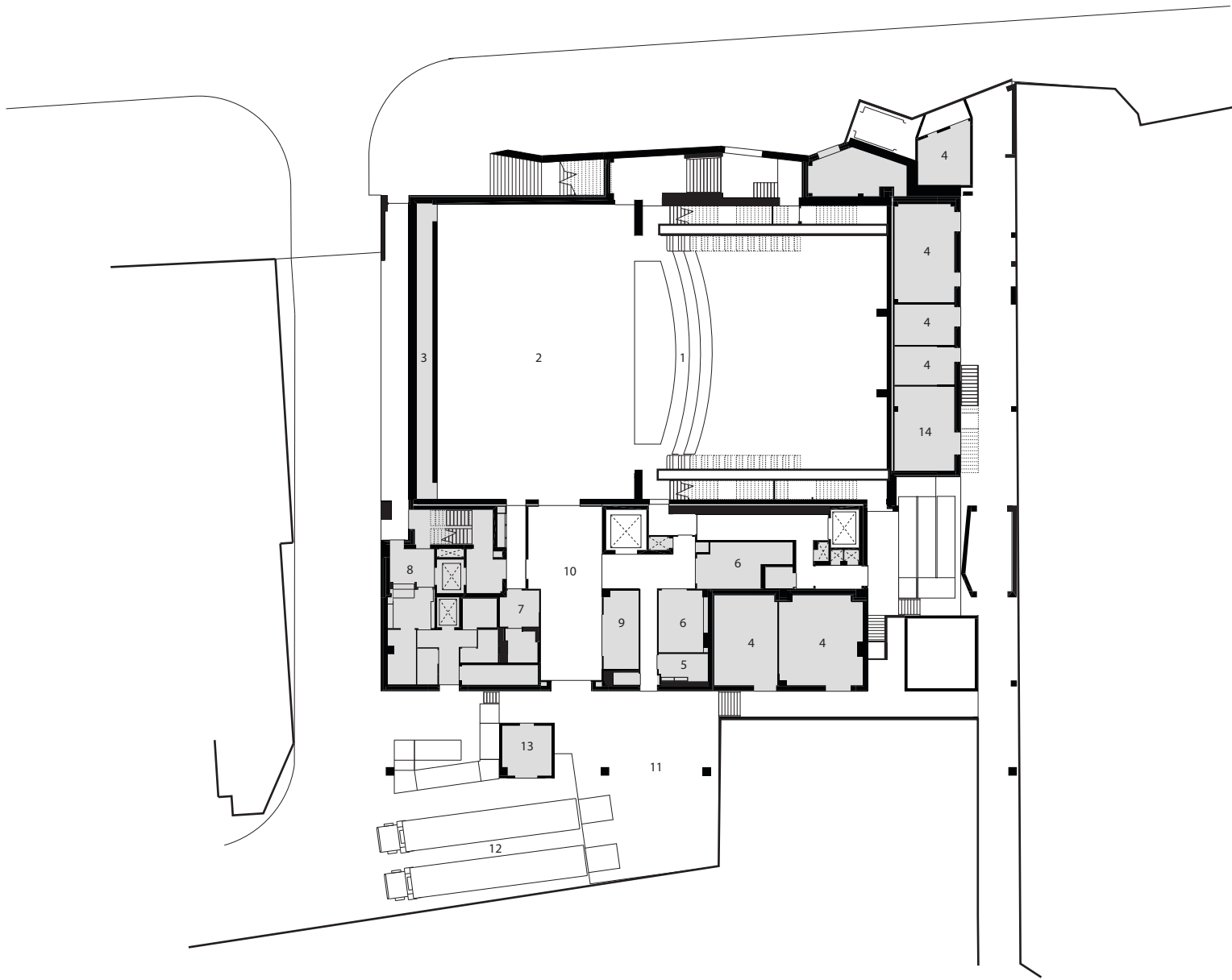
Level -02 Plan (Stage Level)
