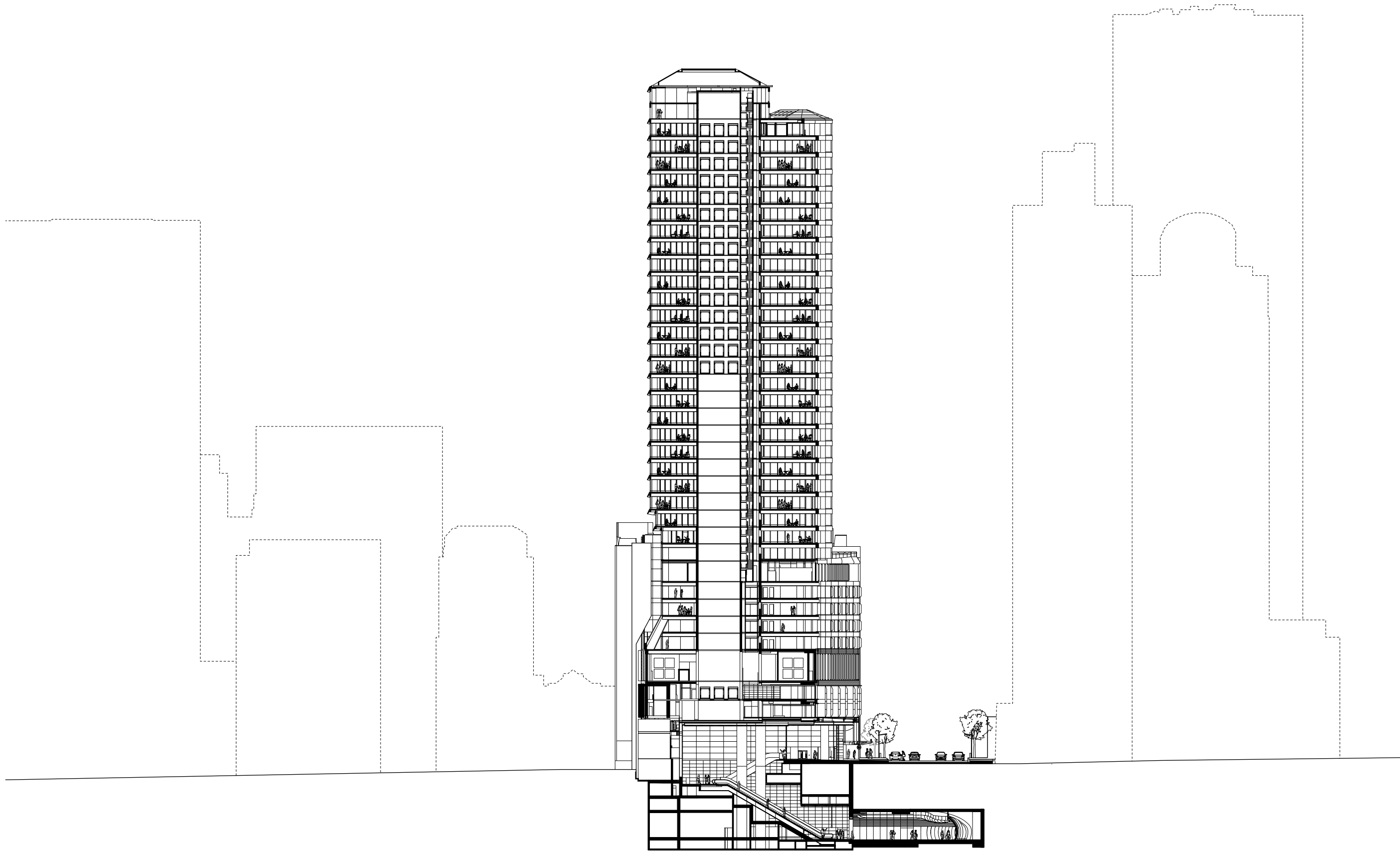
Parkline Place Tower - North South Section
