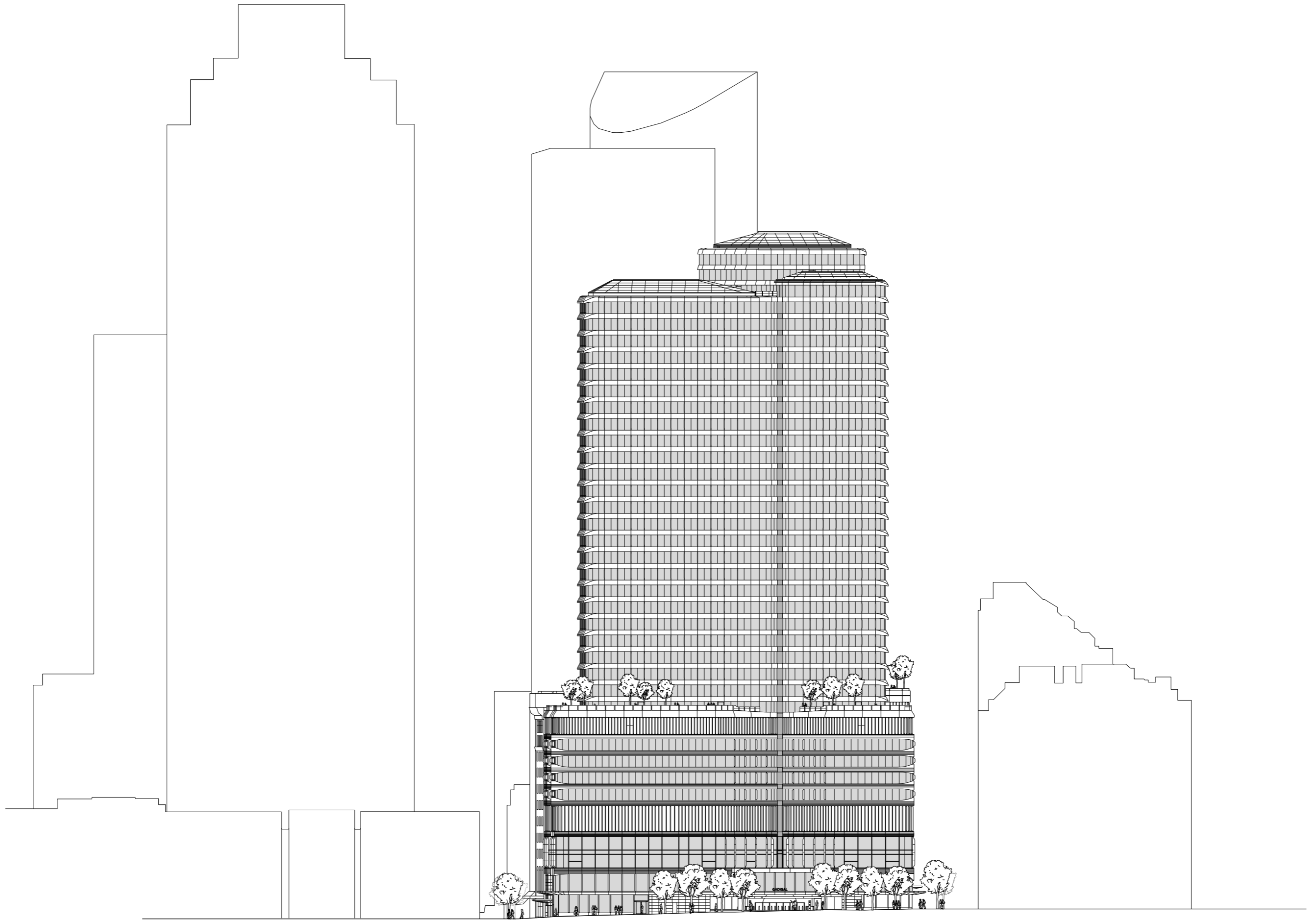
Parkline Place Tower - South Elevation
