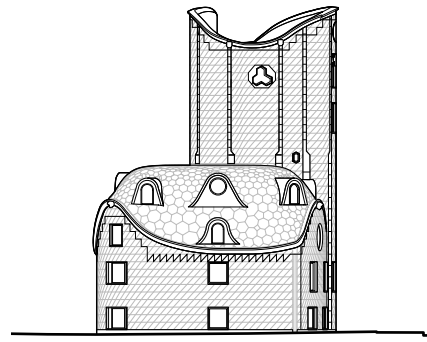
West Elevation
