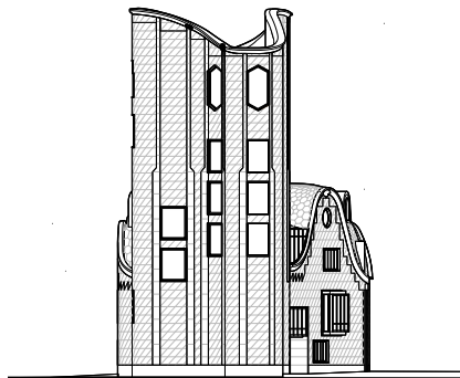
East Elevation
