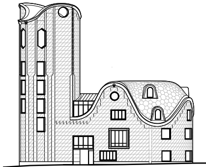
North Elevation
